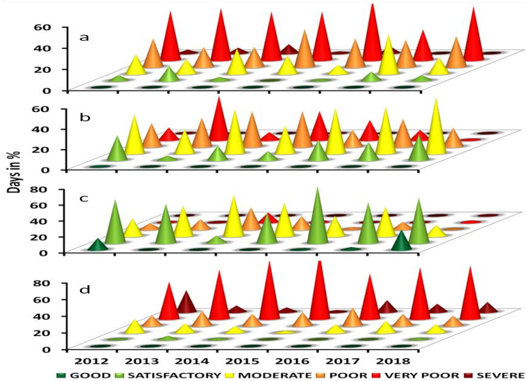
Fig.4: The % variations of days in the year of Air Quality Index during the different seasons (a) winter (b) pre-monsoon (c) monsoon d) post-monsoon during the study period
